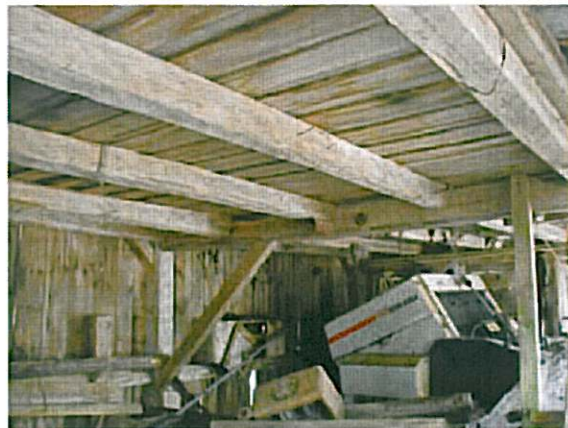
5) Lower level: the floor joists
