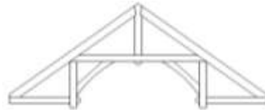
Hammer Beam
